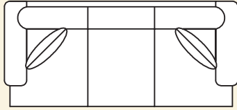
5900 Sofa Overall: H 39 W 84 D 38 Seating: H 18 W 68 D 22 Seat Height: 21 Arm Height: 24 Pillows: 2 P21
