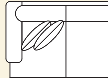
5972 LAF One Arm Loveseat 5973 RAF One Arm Loveseat Overall: H 39 W 53 D 38 Seating: H 18 W 45 D 22 Seat Height: 21 Arm Height: 24 Pillows: 2 P21
