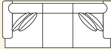
5995 Large Sofa Overall: H 39 W 90 D 38 Seating: H 18 W 74 D 22 Seat Height: 21 Arm Height: 24 Pillows: 4 P21
