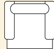
5901 Chair Overall: H 39 W 41 D 38 Seating: H 18 W 24 D 22 Seat Height: 21 Arm Height: 24
