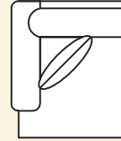
5912 LAF One Arm Chair 5913 RAF One Arm Chair Overall: H 39 W 32 D 38 Seating: H 18 W 24 D 22 Seat Height: 21 Arm Height: 24 Pillows: 1 P21
