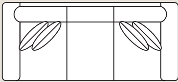
7400 Sofa Overall: H 38 W 90 D 40 Seating: H 18 W 72 D 24 Seat Height: 20 Arm Height: 26 Pillows: 4 P21
