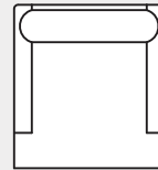
3301 Chair Overall: H 37 W 34 D 38 Seating: H 18 W 24 D 21 Seat Height: 20 Arm Height: 25
